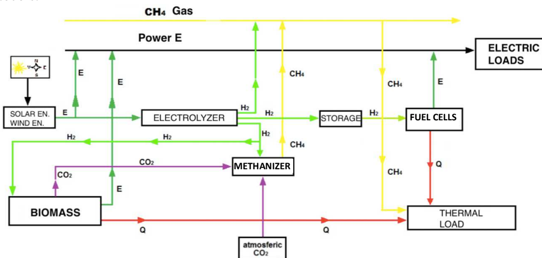
Figure 1: HORESEC Configuration
