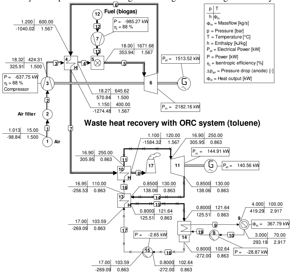
Figure 2. CycleTempo simulation of biogas-fueled gas turbine combined with ORC system.
