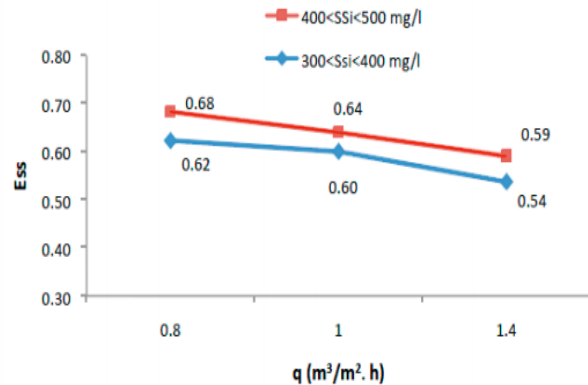
Figure 3: Efficiency at Different SSi Ranges [8]
