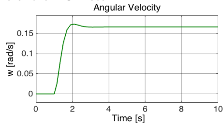
Figure 4: Angular velocity
