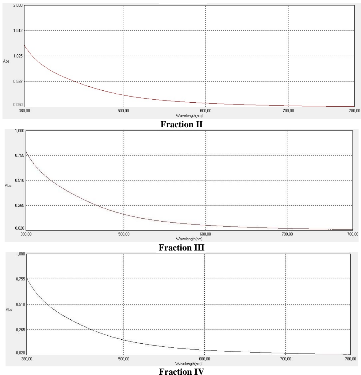
Figure 5 - Spectrograms with dilution 1/1000 in water for nettle fractions
