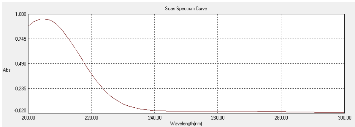
Figure 2: UV absorption spectra of ozonated water after 5 min
