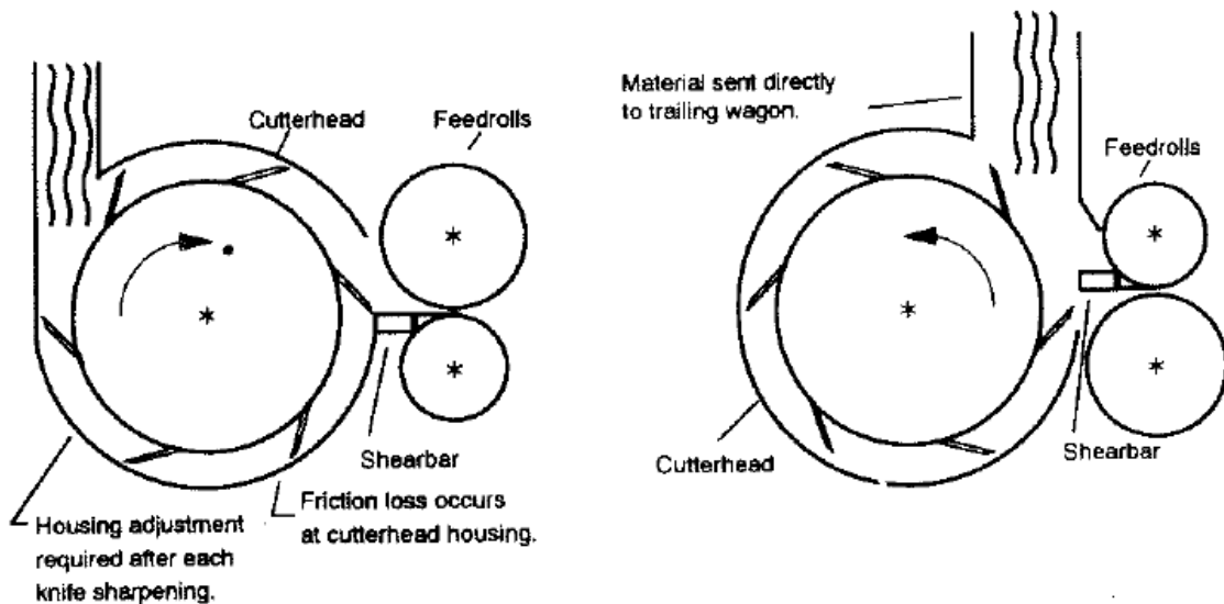
Conventional downward cutting cutterhead Experimental upward cutting cutterhead
