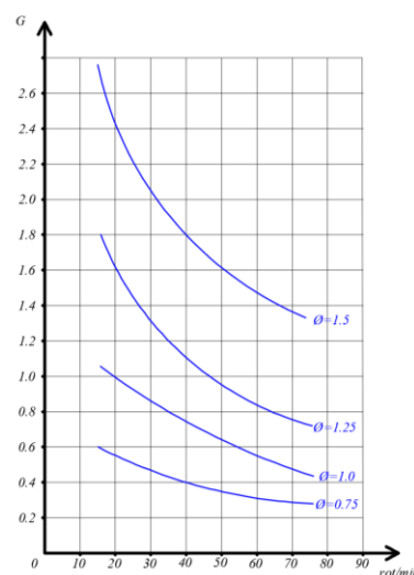
Figure 2: Variation of the degree of feeding the distribution disc depending on the disc orifice diameter and by its rotation speed for bell pepper crop
