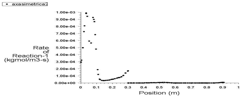
Rate of Reaction-1 ANSYS Fluent Release 16.0 (3d, pbns, spe, rke) Dec 04, 2017 Figure 4. Reaction rate for gypsum forming after asymmetrical axis 2
