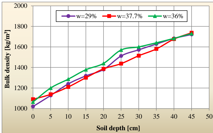
Figure 2: Variation of bulk density with soil depth at different moisture content
