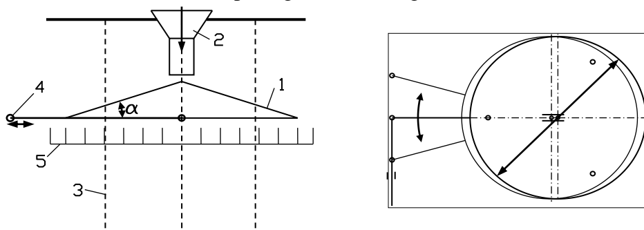
Fig.1. Scheme of suspended conical sieve used in experiments (views at 90^\circ )
