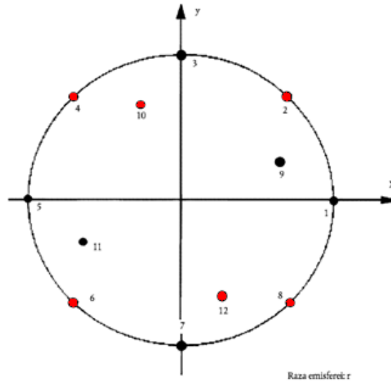
Fig. 2 - Microphone positions for hemispherical measurement surface with 6 microphones [7]
