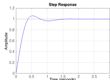
Figure 11: The system response to step command with PID tuned controller
