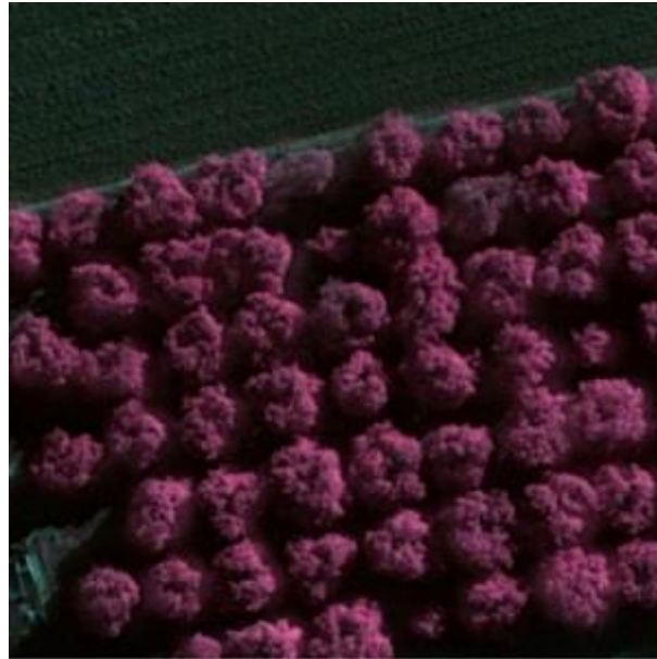
Figure 4: Image analysis [13]
