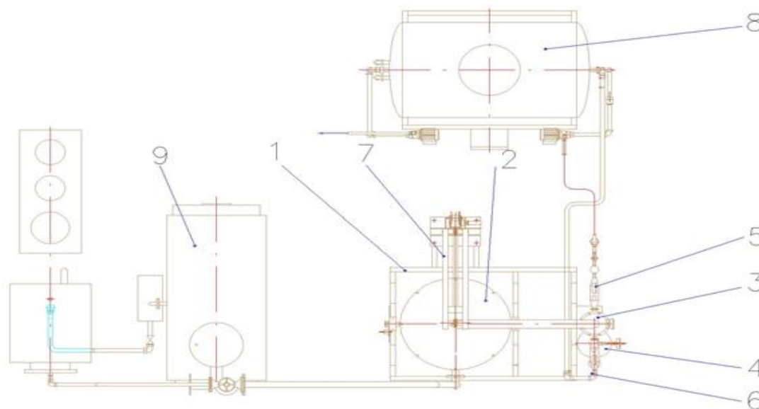
Figure 3: The composition of the steam distillation plant for the extraction of volatile oils
