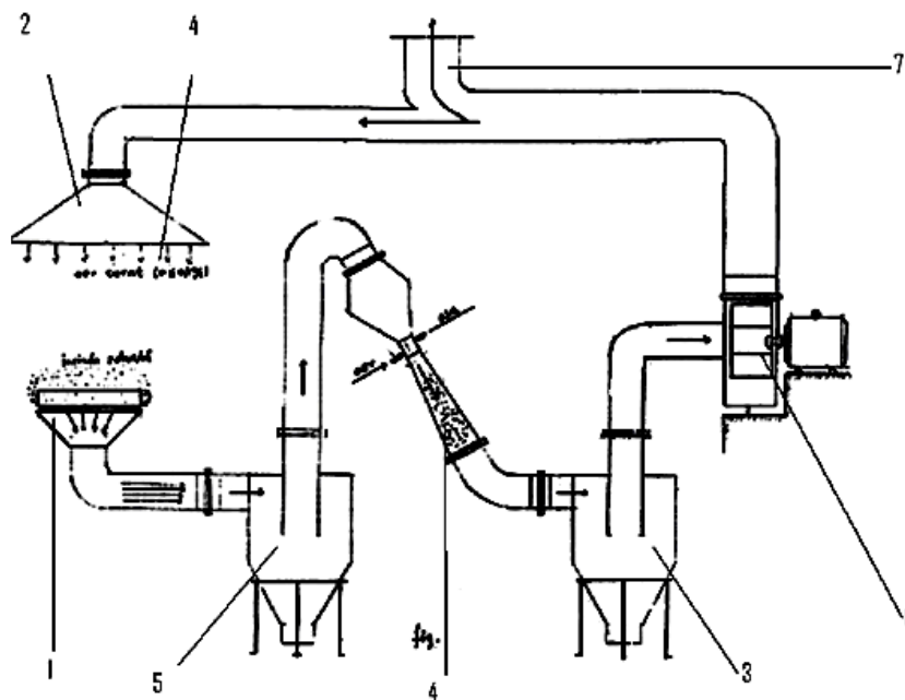
Figure 1: Vacuum cleaner for industrial dust
