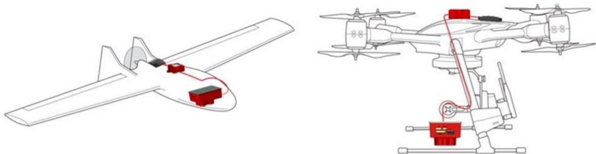
Figure 1: Integrated a multispectral sensor on fixed wings drones or on multi-rotor drones
