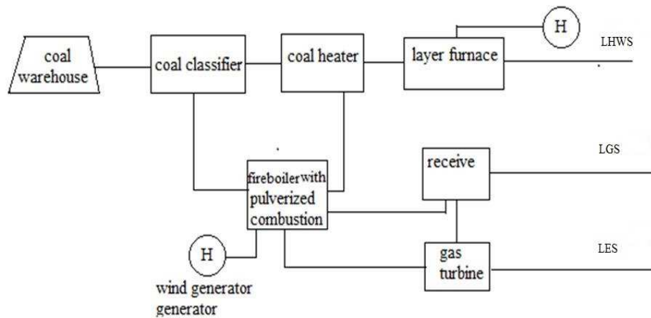
Figure 1: Technology of providing and isolated villages with various types of energy.
