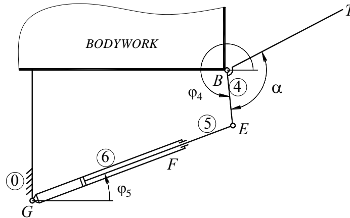
Fig. 7. Definition of the position kinematic parameters of the mechanism (folding phase)
