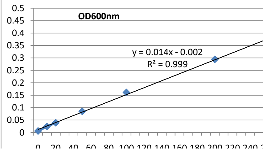
Figure 2: Glucose calibration curve
