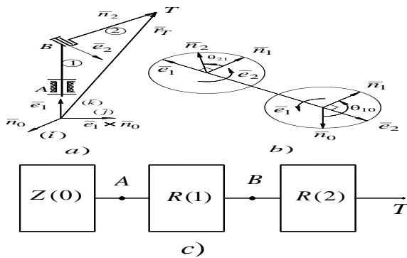
Fig. 1. Manipulator with two degrees of mobility
