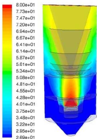
Figure 9: Temperature field on the vertical section ( ^{\circ}\text{C} )
