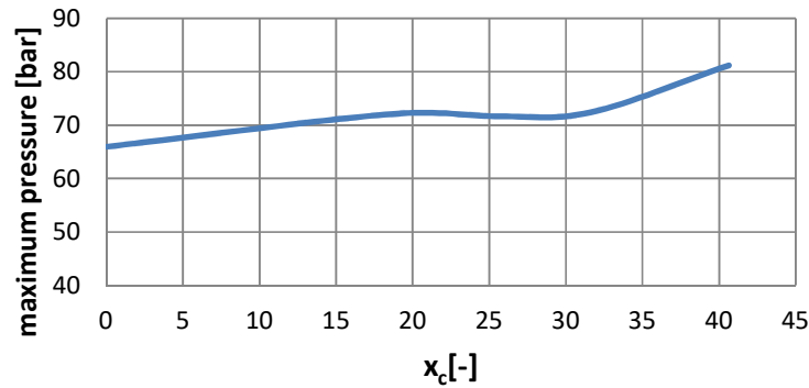
Fig. 1. The maximum in-cylinder pressure.
