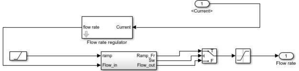
Figure 3: Flow rate regulator
