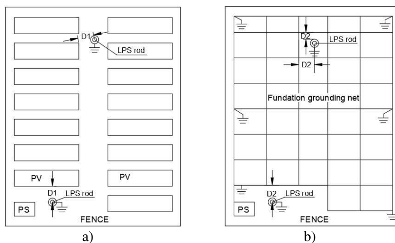
Figure 1: Similar distribution of the ESE lightning rods into the PV panels area in one PVS with insolation distances ( D_1 ) (a). Insolation distances ( D_2 ) of the LPS rods from the closest points of the main element of the earthing system – foundation grounding net (FGN) (b).
