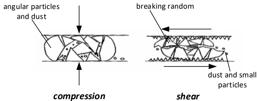
Figure 1: Grinding of wheat seeds with low moisture content (dry), [20]
