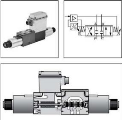
Figure 1: Proportional Directional Control Valve [14]
