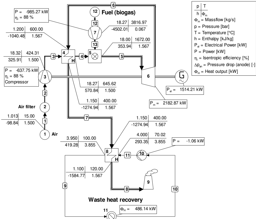
Figure 1. CycleTempo simulation of biogas-fueled gas turbine cogeneration system.
