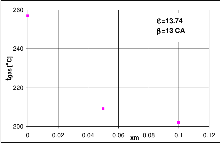
Figure 2: The gas temperature versus animal fats content
