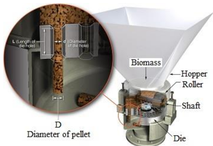
Figure 5: Schematic showing expansion of the high moisture pellet during compression and extrusion in a flat die pellet mill [18]
