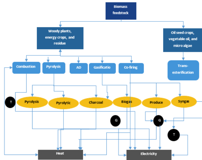
Biomass to energy pathway
