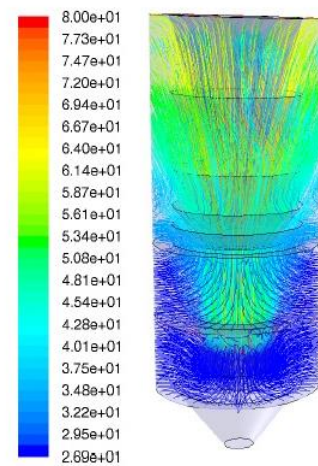
Figure 11: Path lines field on the vertical section [8]
