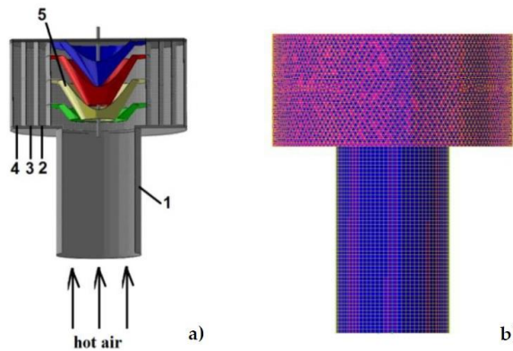
Figure 5: Geometry of driers and deflectors: a) section; b) hybrid mesh (1 thermal agent pipe (hot air), 2 layer I of seeds, 3 layer II, 4 layer III, 5 deflectors) [7]
