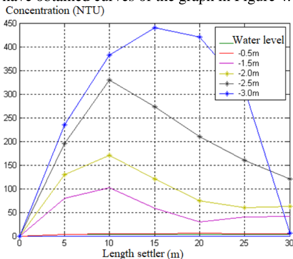
Figure 4: Changes in concentration depending on the length of the settling tank to different depths [9]
