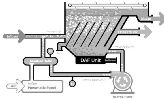
Figure 2: Dissolved air flotation systems [5]
