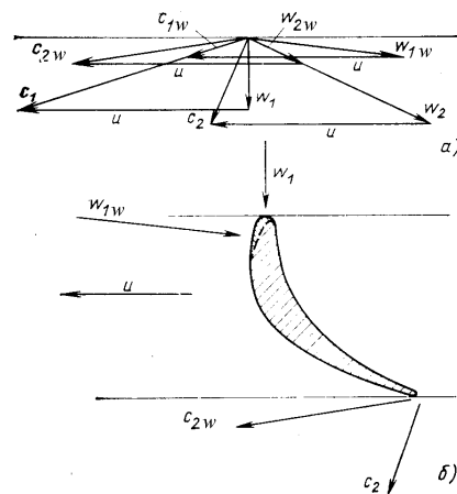
Figure 2. Velocity diagrams for wet steam (index w – water droplets)
