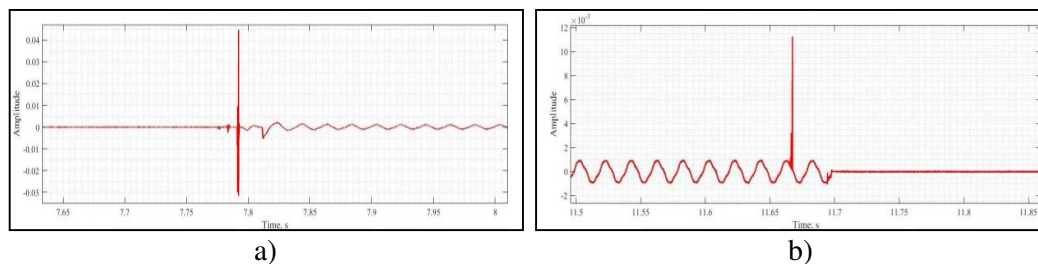
Figure 4: The moment of switching the load Tr.AL2 on (a) and off (b). Experiment №2
