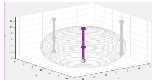
Fig. 4. Total workspace
