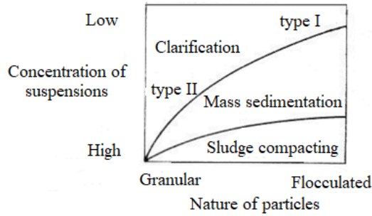
Figure 1: Decantation phases [5]
