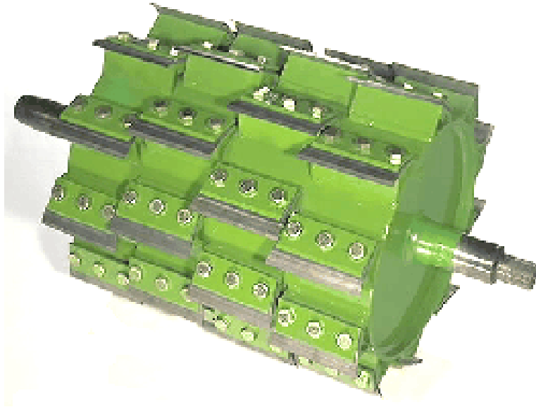
Figure 6: John Deere 800 Series chopping drum [6]
