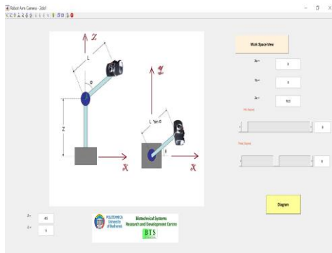
Fig. 3. Simulation program interface of the camcorder manipulation arm kinematics
