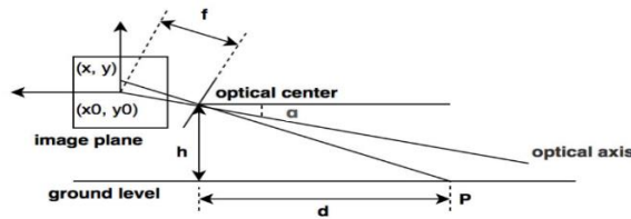
Fig. 7. The geometric pattern of distance detection from an object
