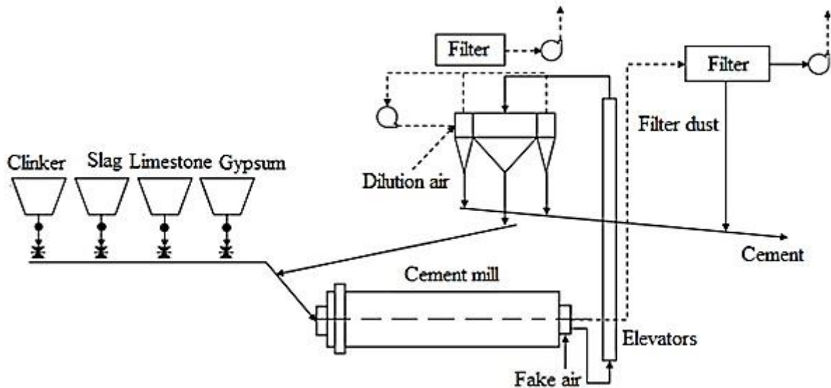
Figure 1: The flowchart of cement grinding [5, 6]
