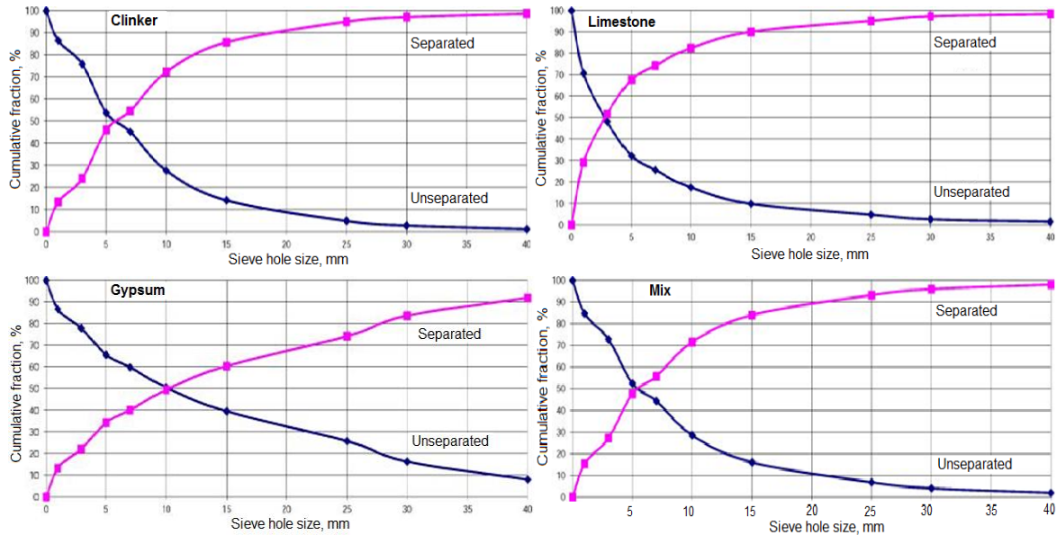
Figure 6. The particle size distribution of the components subjected to grinding for cement manufacture
