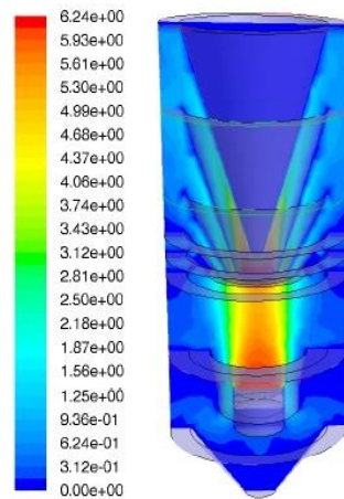
Figure 10: Velocity field on the vertical section ( \text{m s}^{-1} ) [8]
