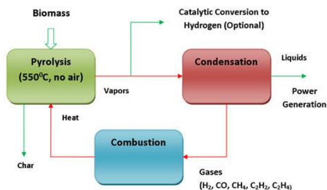
Figure 2 Process conditions for pyrolysis of biomass [3]
