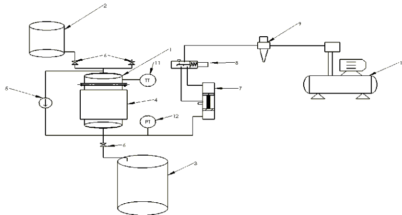
Figure 1. Principle diagram of the equipment for obtaining organic biofertilizers / bio-insecticides – EXTBIO (1-extraction vessel, 2-loading charging tank, 3 – final product unloading tank, 4-heating mantle with thermostat, 5-recirculation pump, 6-electro-valves, 7-double piston cylinder, 8- pneumatic distributor, 9-pressure regulator, 10 – compressor, 11 – Pt100 thermo-resistance, 12 – pressure transducer)
