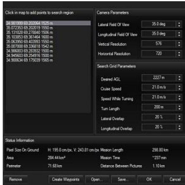
Figure 2: Flight planning [13]
