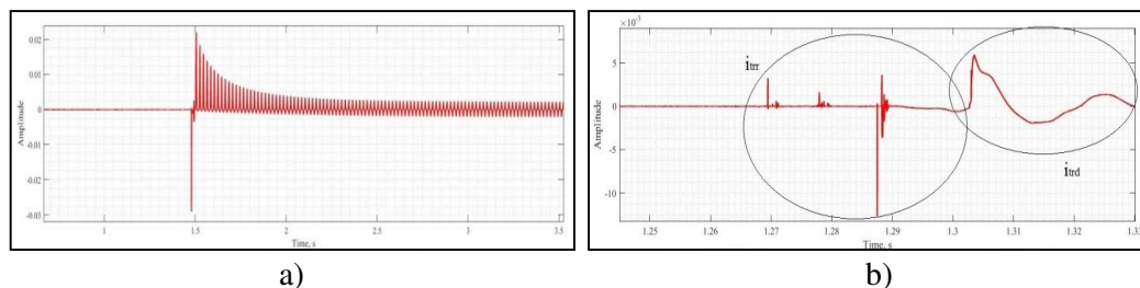
Figure 3: The moment of the switching the load Tr.AL1 on. Experiment №1(a). The both components of the i_{tr}(t) : i_{irr}(t) and i_{ird}(t) in the current timing diagram (b).
