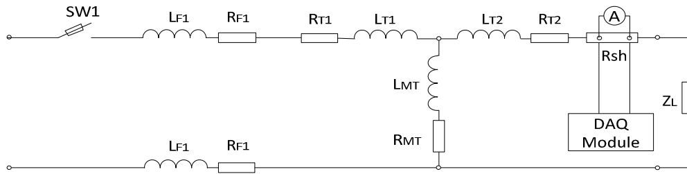
Figure 1: Equivalent circuit of the system “power supply transformer – feeder – load”. Point of commutation for experiments № 1 and 2 – SW1
