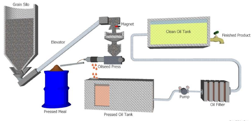
Figure 4: Small scale oilseed pressing process[6]
