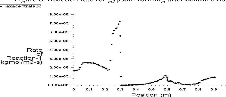
Rate of Reaction-1 ANSYS Fluent Release 16.0 (3d, pbns, spe, rke) Dec 04, 2017 Figure 7. Reaction rate for gypsum forming after central axis 3c
