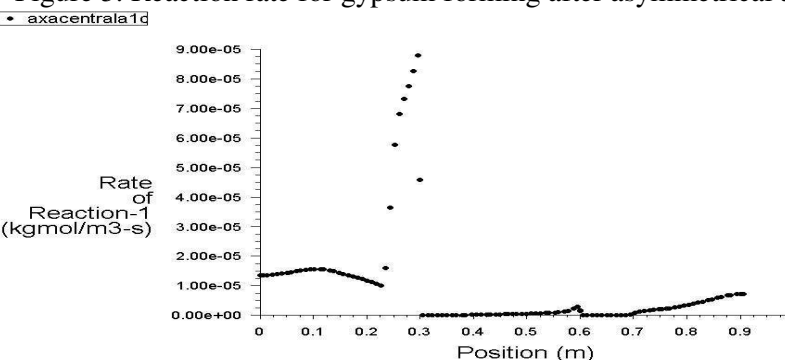
Rate of Reaction-1 ANSYS Fluent Release 16.0 (3d, pbns, spe, rke) Dec 04, 2017 Figure 6. Reaction rate for gypsum forming after central axis 1c
