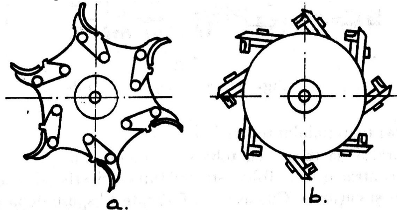
Figure 1: Chopping drums [1]
